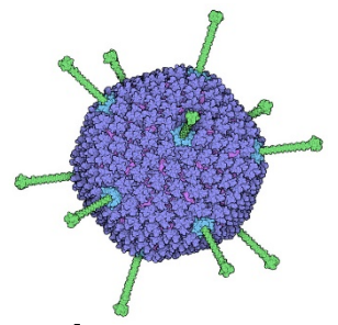
adenovirus 0.1 \mu\text{m}
