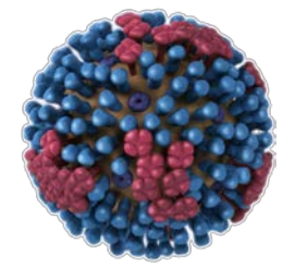
influenza 0.1 \mu\text{m}
